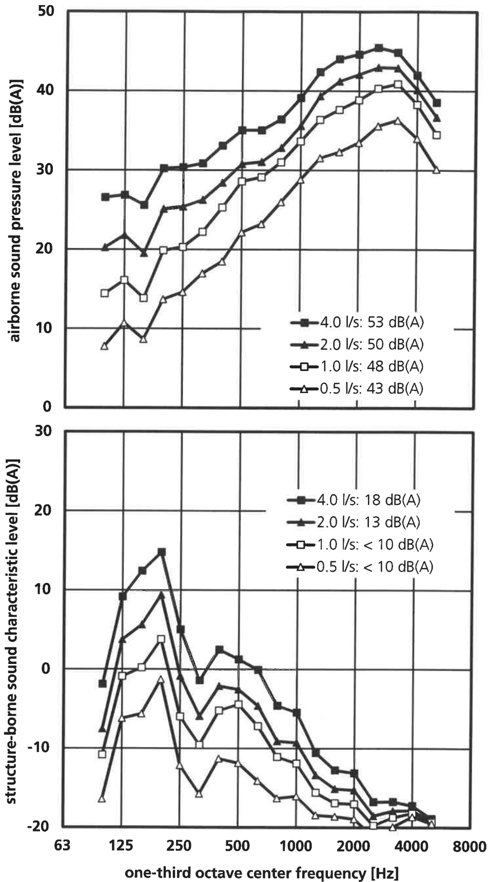
Frequency spectrum of the airborne sound pressure level L_{a,A} (above) and structure-borne sound characteristic level L_{sc,A} (below) measured at various flow rates according to EN 14366. Test specimen: Wastewater installation system "DIZAYN, Nanotek 110x3.4" (manufacturer: Dizayn). The wastewater system consisted of straight plastic pipes and fittings and acoustic pipe clamps (double clamps) "DIZAYN, 120" (supporting and guidance clamp) and "DIZAYN, 110, 105-112" (fixing clamp).
